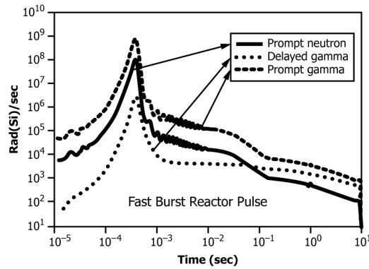
NOTE 1—Fig. 2 shows the radiation components from a maximum pulse [ \Delta\Theta = 300^\circ\text{C} , neutron fluence = 3.4 \times 10^{14} 1-MeV(Si)/ \text{cm}^2 ] in a fast burst reactor. The wiggles in the millisecond time period are a real effect and represent the temperature-induced shock oscillations in the reactor power as a result of the fuel expansion. The time-dependence of the reactor pulse was measured with a diamond PCD and the calculations were performed to deconvolute the radiation components of the reactor pulse (11,12).
