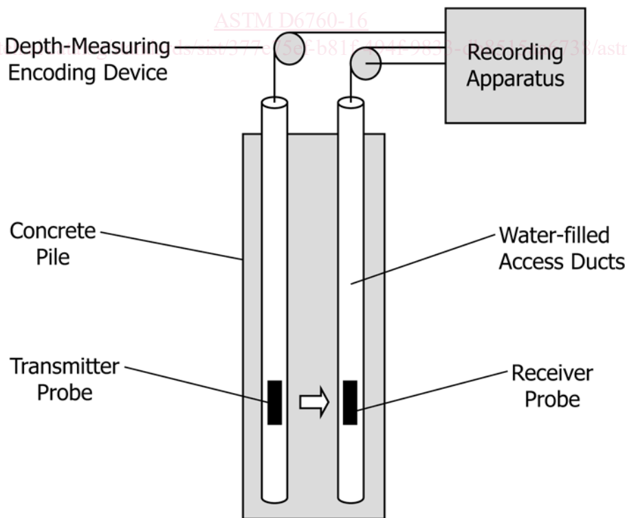
FIG. 3 Test Arrangement
