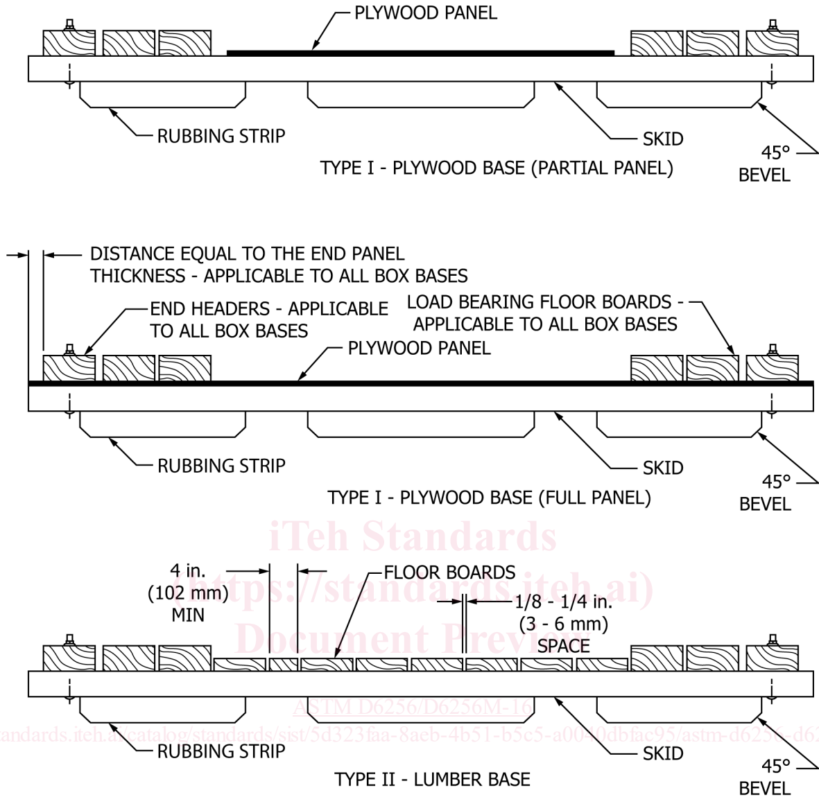
FIG. 1 Base Types
