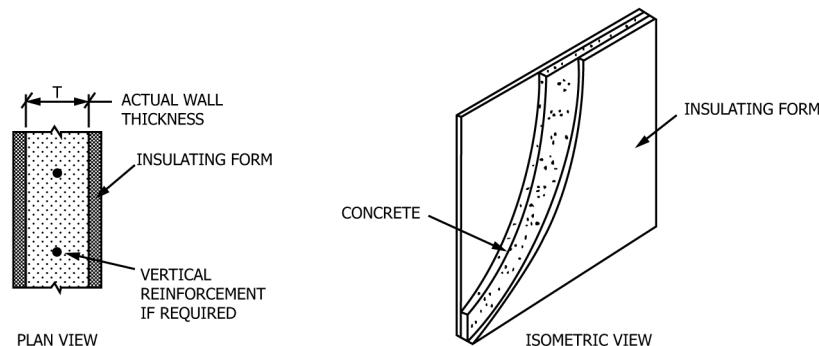
FIG. 1 Flat Wall ICF, Wall Assembly
