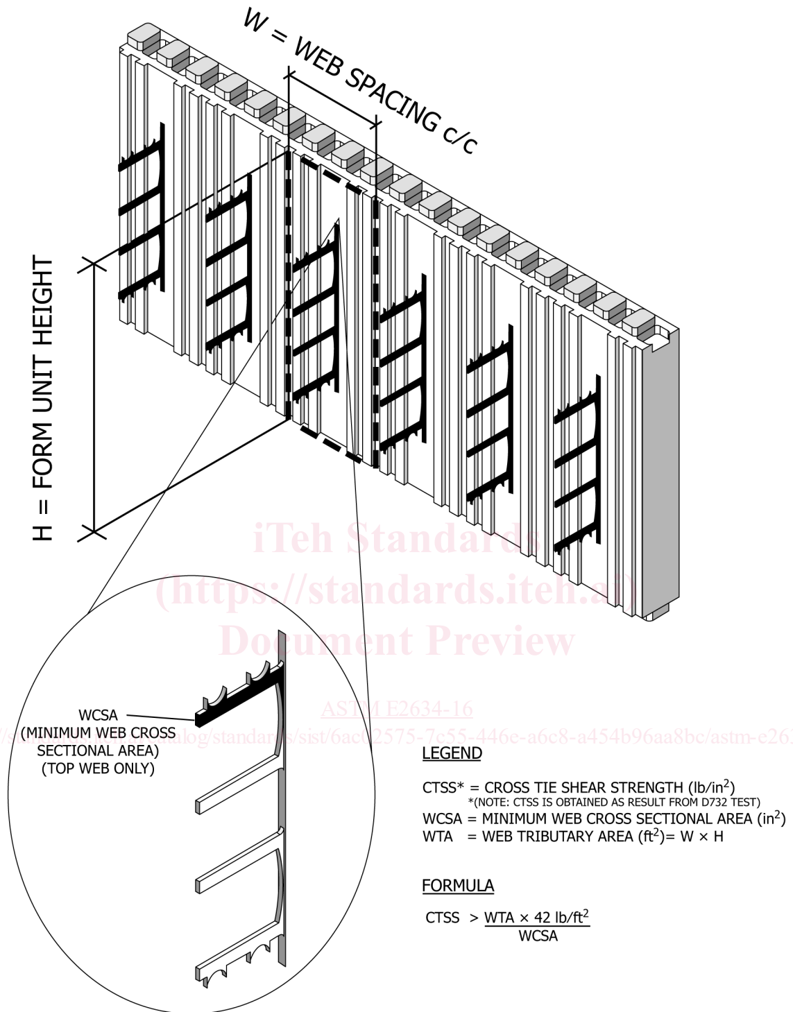
FIG. 2 Tributary Areal Associated with the Web Cross Sectional Area that would be Subjected to the Shear Strength
