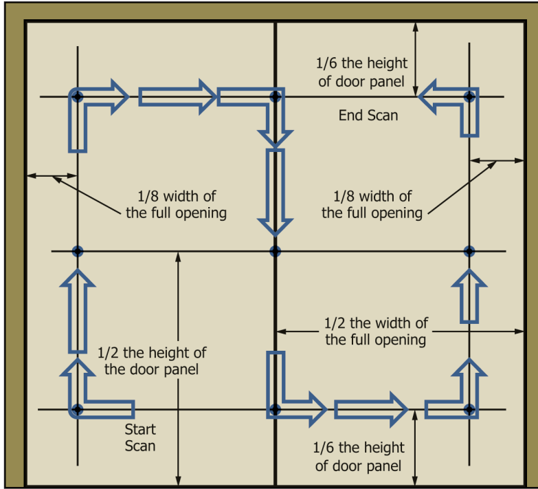
FIG. 2 Microphone Locations for Opening More than One Meter Wide with Scan Pattern
