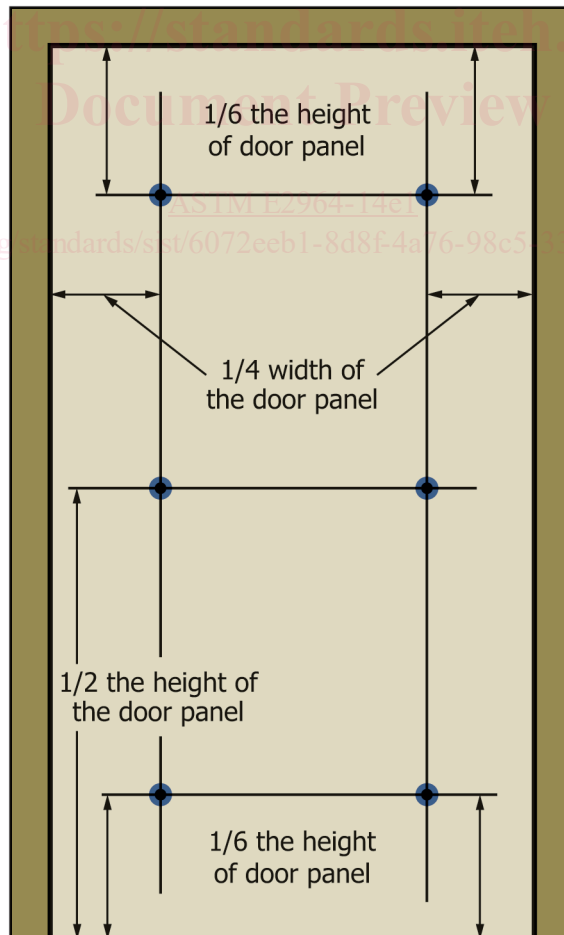
FIG. 1 Microphone Locations for Opening 1 m or Less Wide
