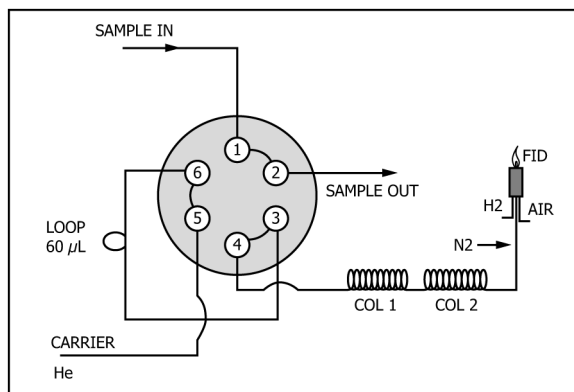
FIG. 2 Valve-On—Injection Direct Valve Injection Sample Introduction: Valve On—Injection
