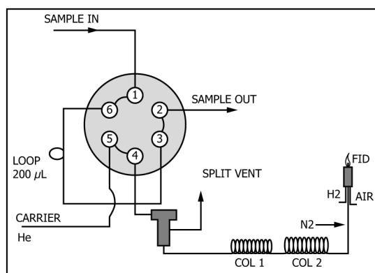
FIG. 3 Split Valve Off—Sample Injection Sample Introduction: Valve Off—Sample Loading
