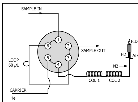
FIG. 1 Direct Valve Off—Sample Injection Sample Introduction: Valve Off—Sample Loading
