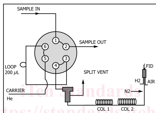
FIG. 4 Valve On—Injection Split Valve Injection Sample Introduction: Valve On—Injection
