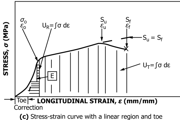
FIG. 4 Examples (a, b, c) of CFCC Stress-Strain Curves
