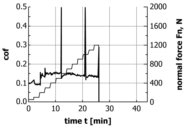
FIG. X1.1 Sample Recording Chart During Step Load Test
