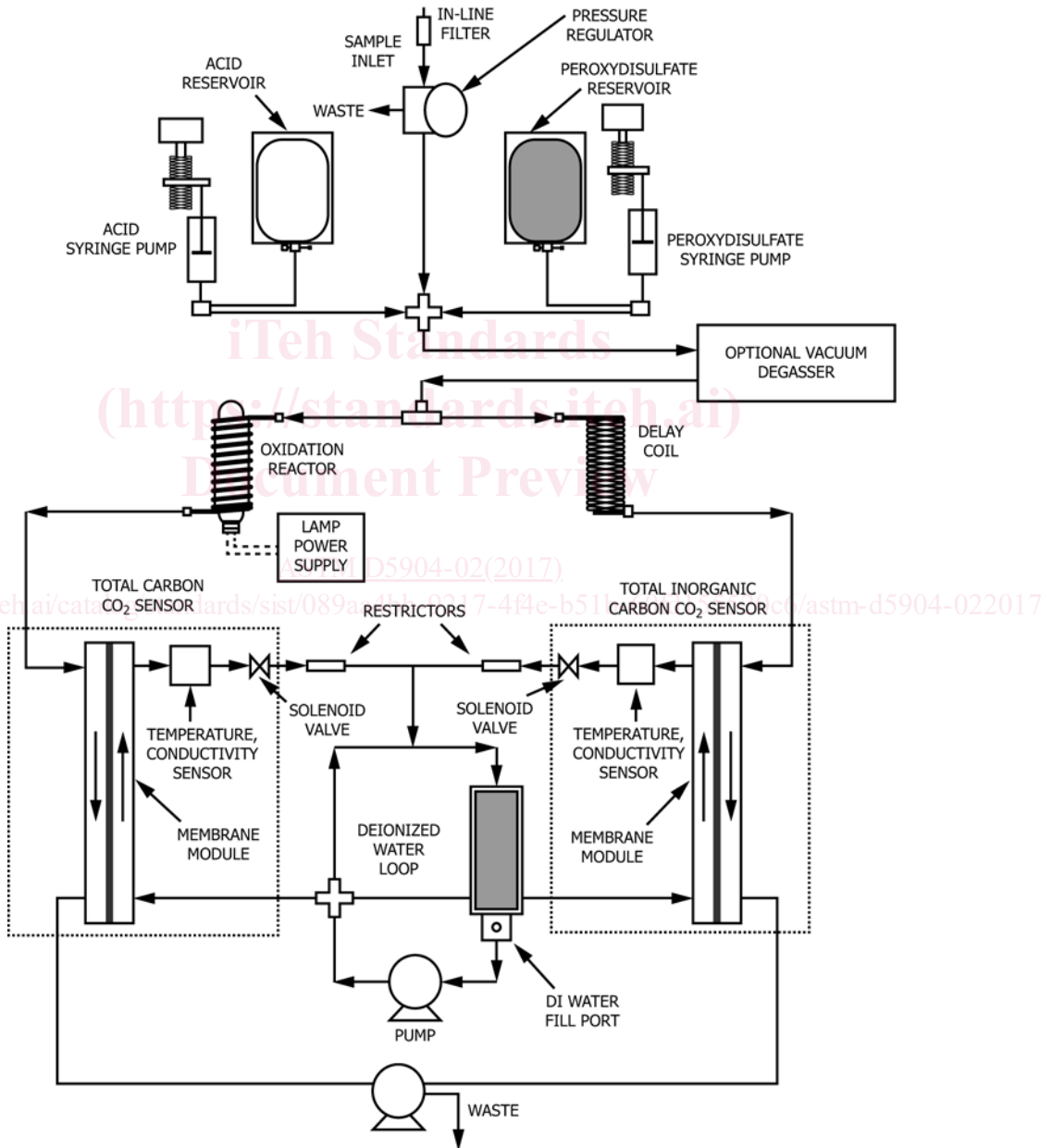
FIG. 1 Schematic Diagram of TOC Analyzer System
