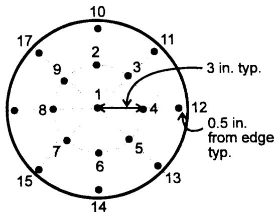
FIG. 1 Thermocouple Placement
