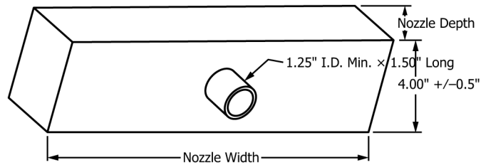
FIG. 1 Nozzle Adapter
