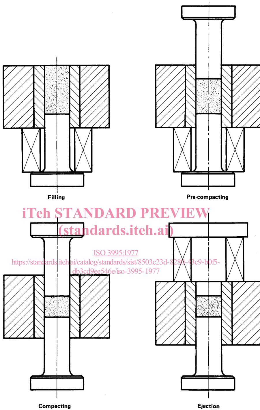
FIGURE 4 – Procedure of compacting and ejection
