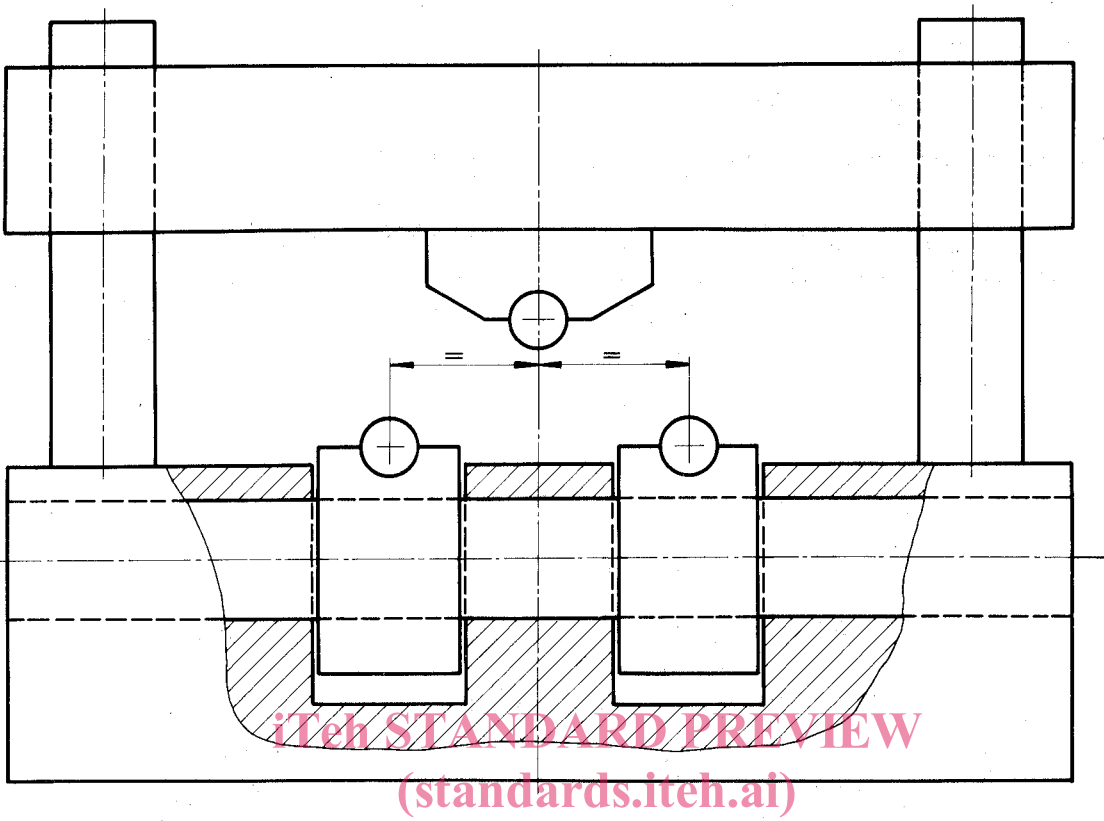
FIGURE 2 – ISO 3995-1977 Diagram of test fixture https://standards.iteh.ai/catalog/standards/sist/8503c23d-8280-43c9-b0f5-db3cd9ee546e/iso-3995-1977
