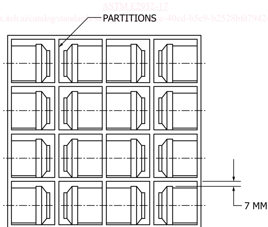
FIG. 1 (a) Vibration Test Device
