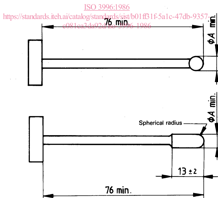
Figure 1 — Gauge plugs for testing constriction of bore of hose 1)
