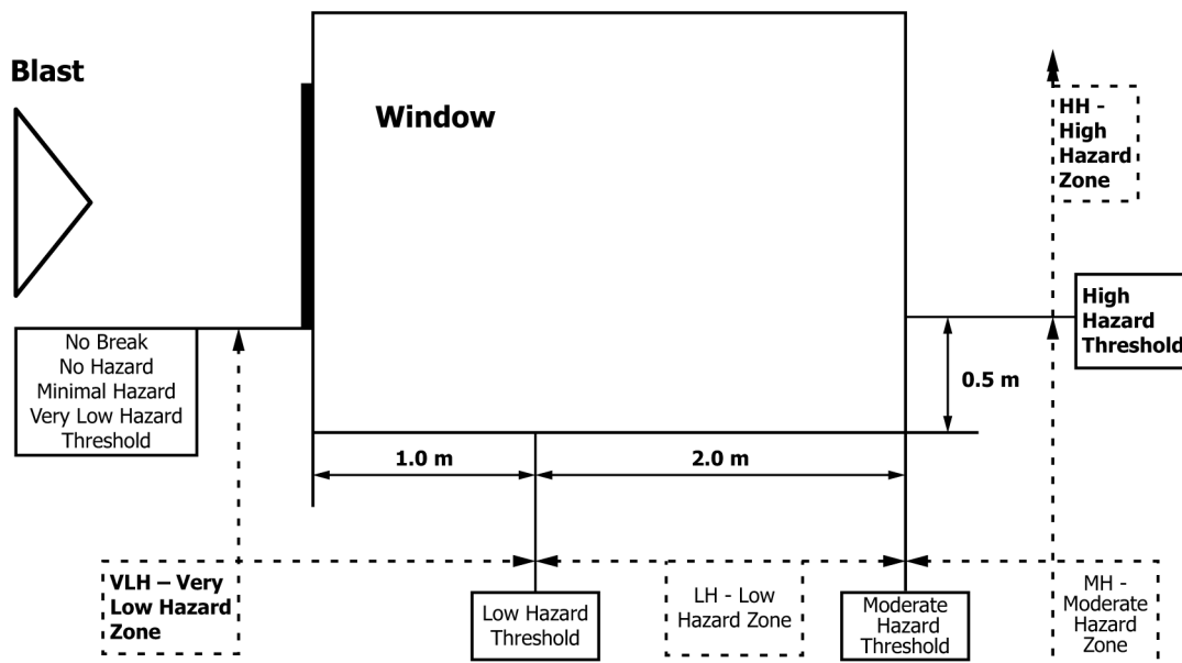
FIG. 1 Cross-Section Cross Section Through Witness Area
