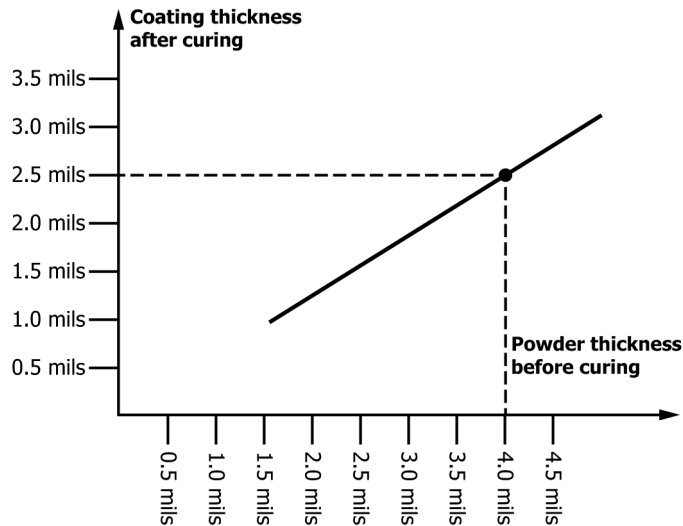
FIG. 1 Typical Correlation Between Pre- and Post-cured Powder
