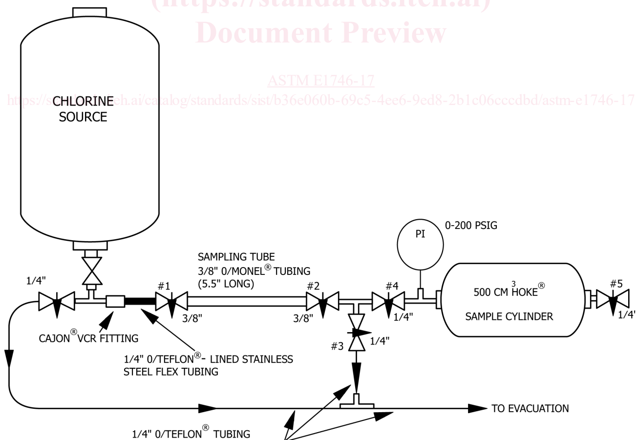
FIG. 2 Chlorine Sampling Apparatus
