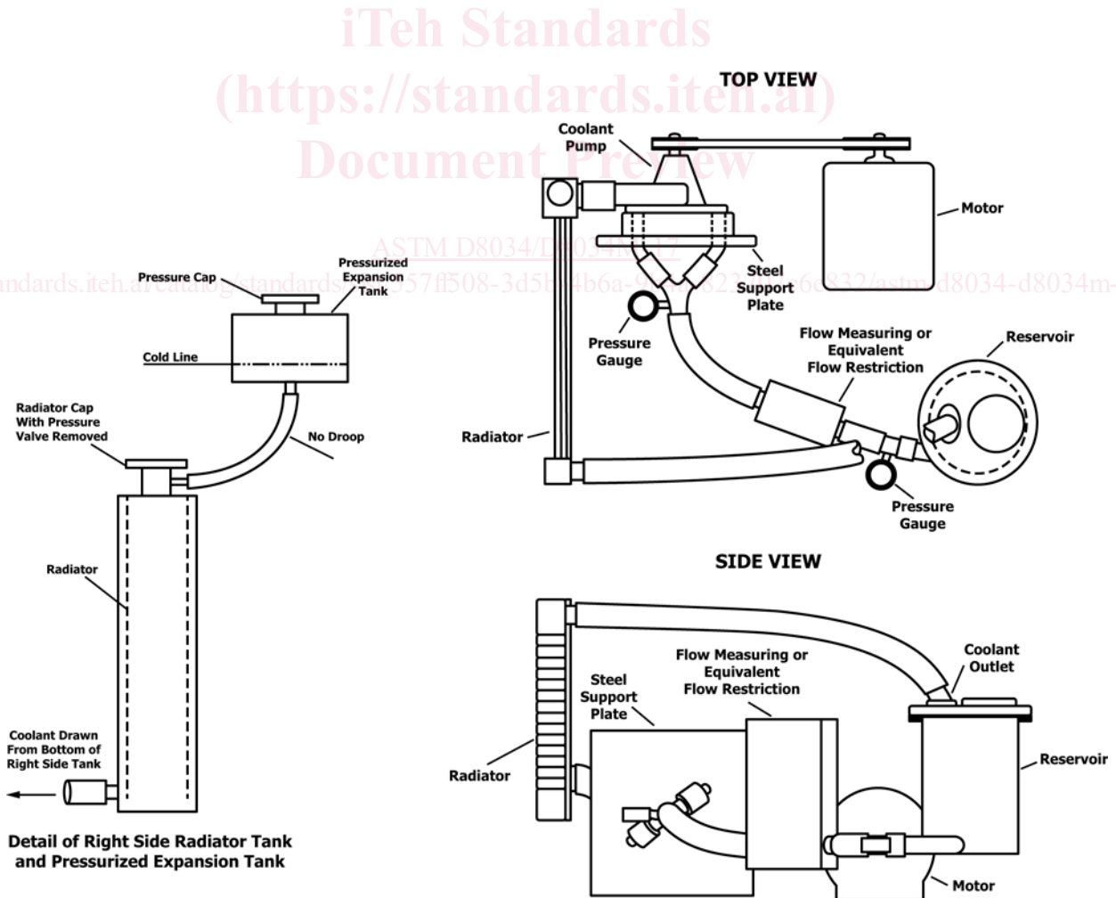
FIG. 2 Assembly of Test Apparatus
