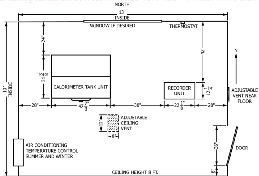
FIG. 4 Calorimeter Room
