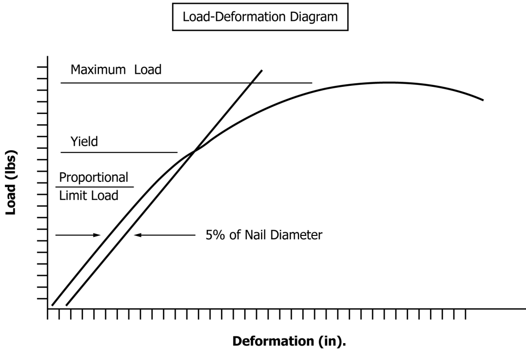
FIG. 21 Example of Typical Load-Deformation Diagram from Nail Bending Test
