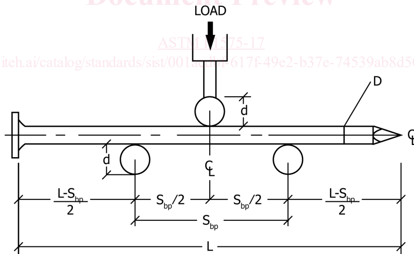
FIG. 12 Center-Point Bending Test for Load and Bearing Point Locations for Smooth Shank and Fully Deformed Shank Nails
