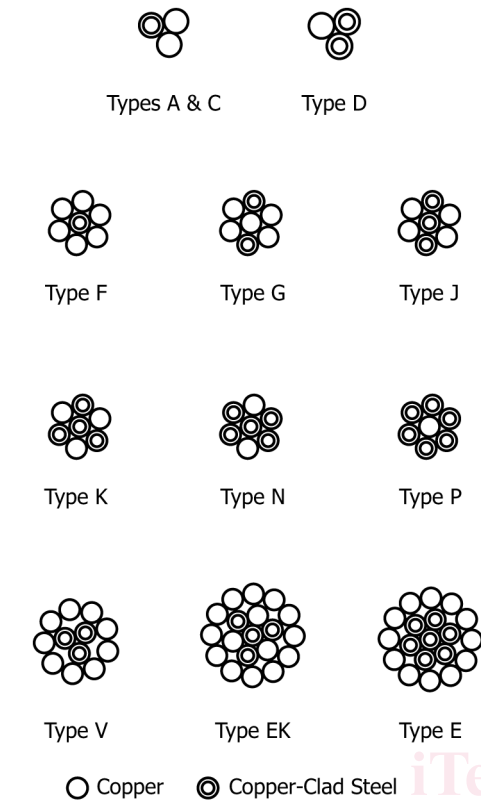
FIG. 1 Standard Types of Composite Conductors
