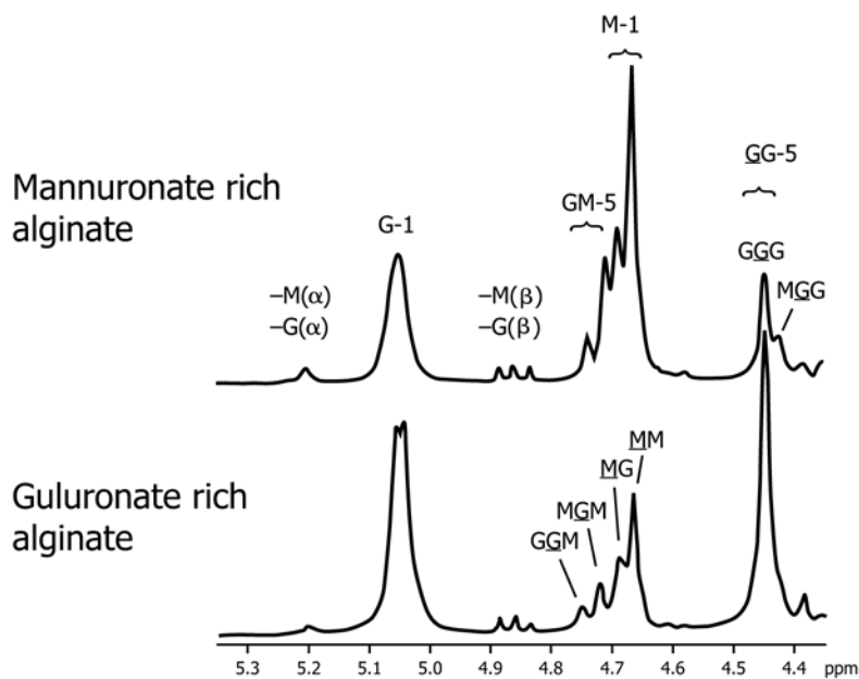
FIG. 2 Typical ^1\text{H} NMR of Sodium Alginate
