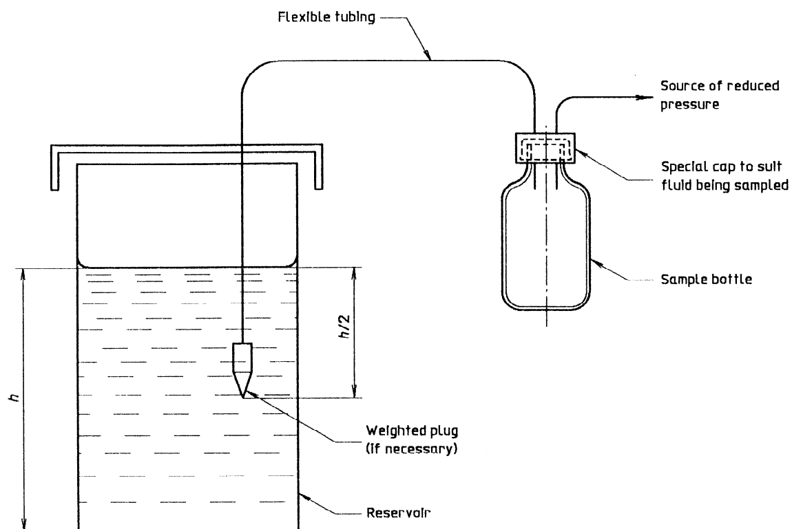
Figure 2 — Typical example of a reservoir sampler (standards.iteh.ai)
