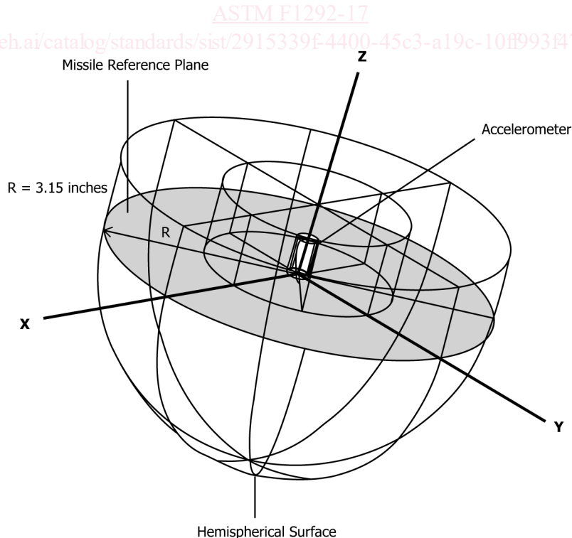
FIG. 1 Missile Reference Plane and Axes
