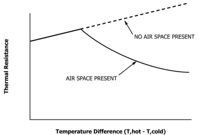
FIG. 1 Schematic of Thermal Resistance for a Permeable Attic Insulation Under Simulated Winter Conditions (Heat Flow Up)
