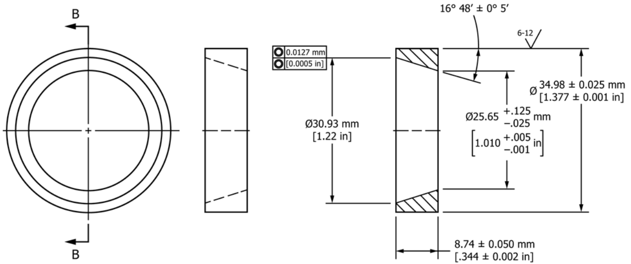
SECTION B-B
