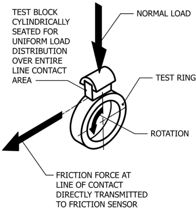
FIG. 1 Test Schematic
