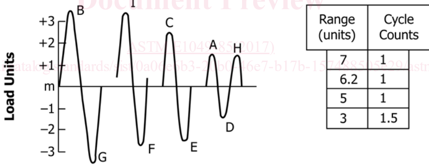
(c)—Cycles Derived from Peak Count of (a)
