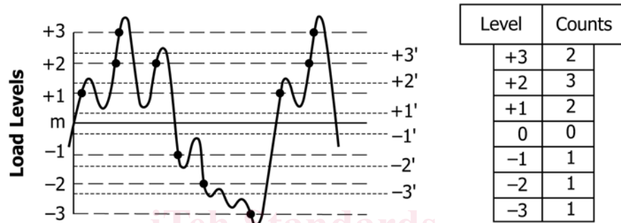
(b)—Restricted Level Crossing Counting
