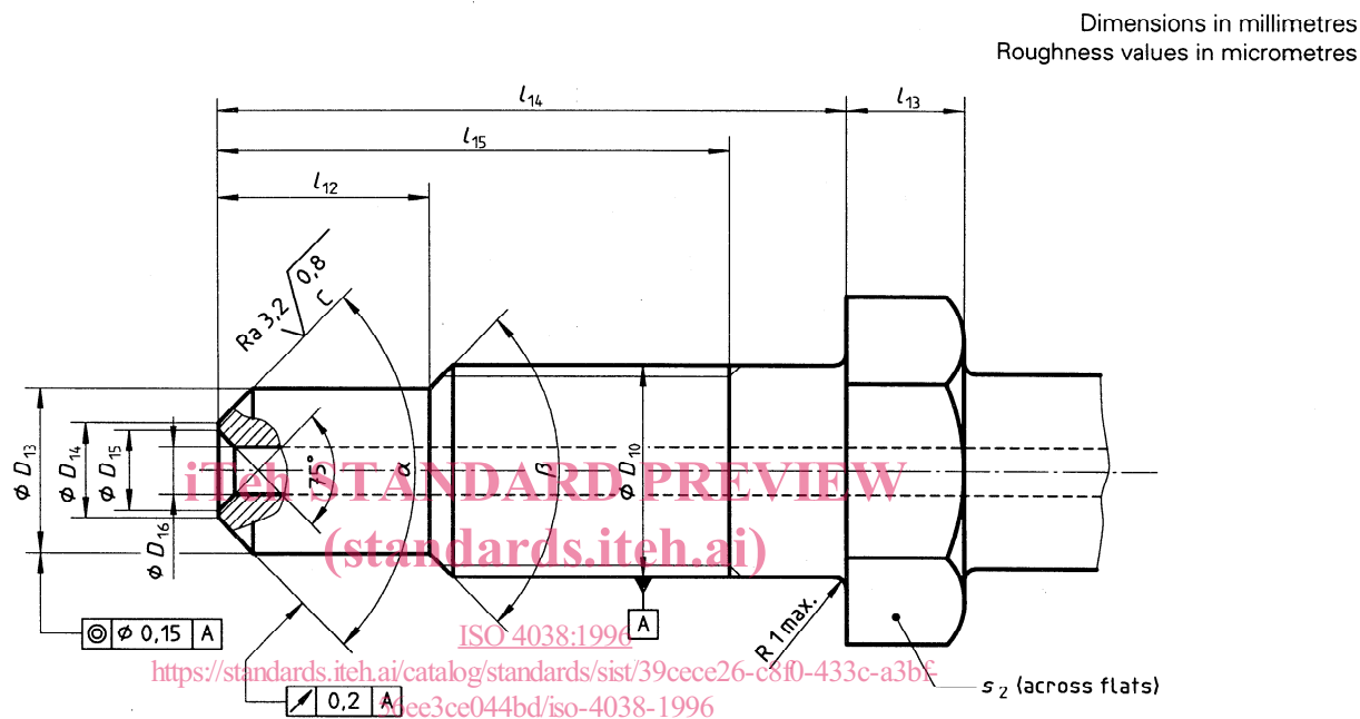
Figure 6 — Male hose end fittings for cone sealings
