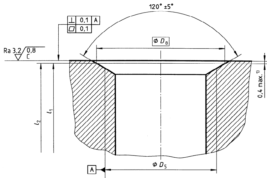
Figure 4 — Optional hole entry
