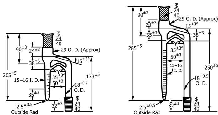
FIG. 1 —TrapsTraps (Style A)
