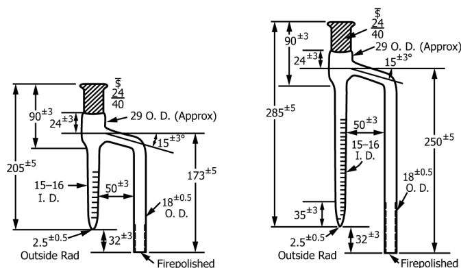
FIG. 3 —TrapsTraps (Style C)
