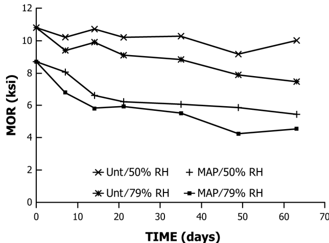
FIG. 2 SYP Southern Pine Plywood Exposed at 170°F (77°C) 77°C (170°F)
