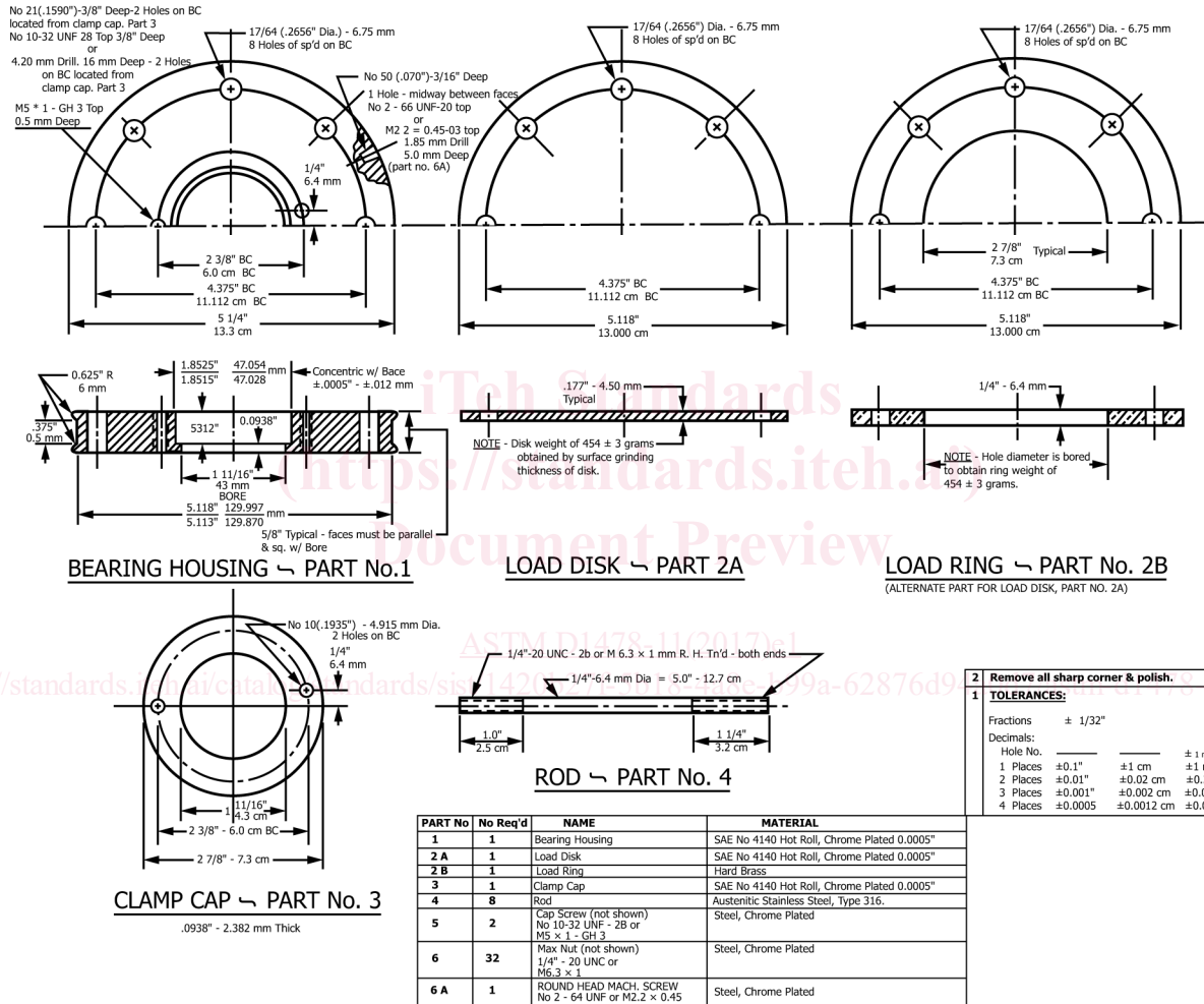
FIG. 3 Cage Parts
