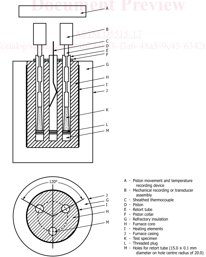
FIG. 2 Typical Dilatometer Apparatus
