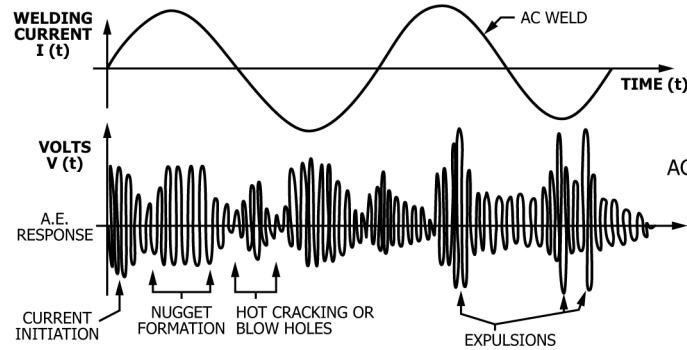
FIG. 2 Typical AE Response Signals During Current Flow
