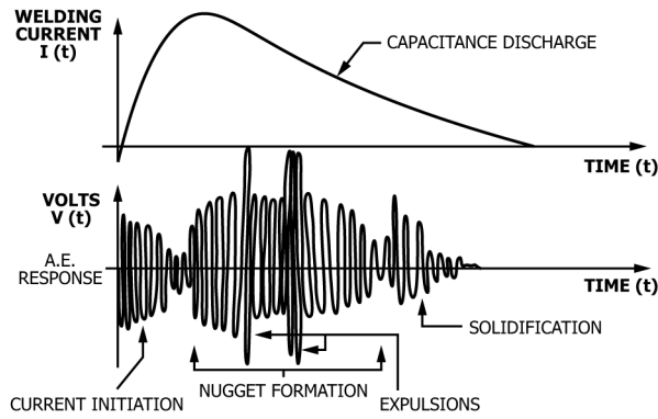
FIG. 2a DC WELDING CURRENT
