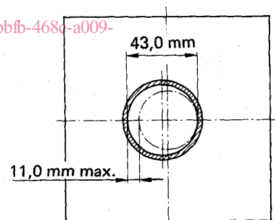
FIGURE 1 — Maximum clearance between centring device and tube
