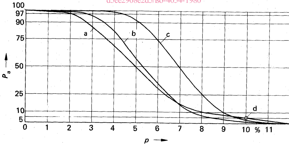
P_a = probability of acceptance p = percent defective a = curve as recommended in 8.2.3.2 b = operating characteristic curve associated with sampling plan L, AQL 2,5 in ISO 2859 c = operating characteristic curve associated with sampling plan M, AQL 4,0 taken from ISO 2859 d = limiting point ( p = 10\%; P_a = 5\% ) as specified in 6.2.2 and 8.2.3.3.
