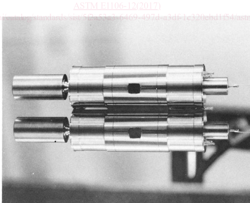
FIG. 4 Photograph of the Capacitive Transducer and its Reflection in the Steel Block
