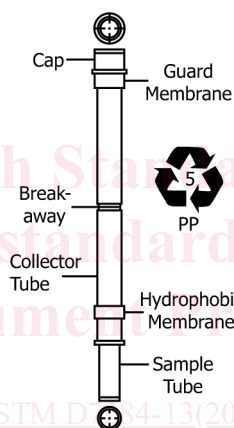
FIG. 2 Micro Distillation Sample Tube
