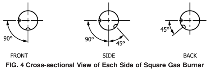
FIG. 4 Cross-sectional View of Each Side of Square Gas Burner
