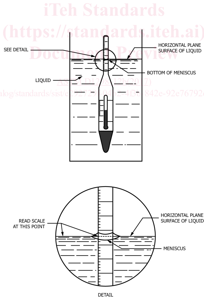
FIG. 1 Hydrometer Scale Reading for Transparent Liquids
