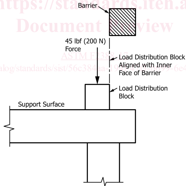
FIG. 34 Stability Test
