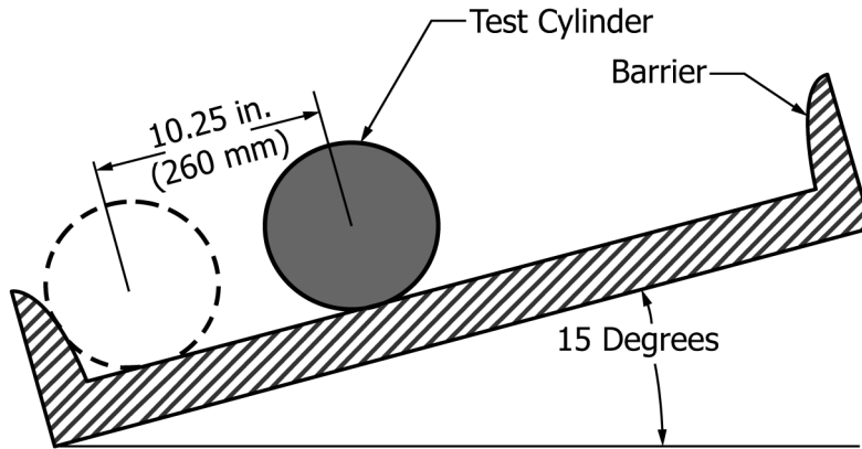
FIG. 45 Barrier Retention Test
