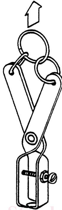
FIG. 23 Tension Test Clamp
