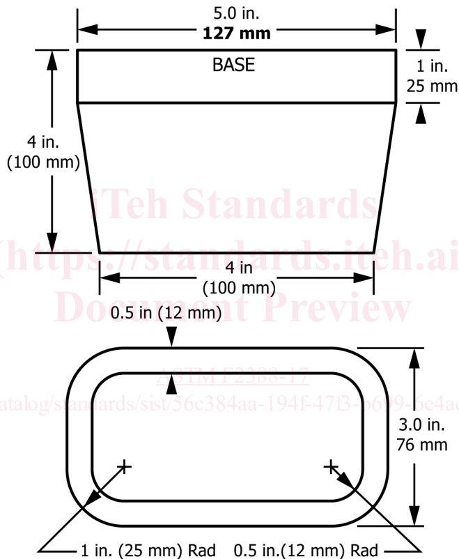
FIG. 45 Barrier Retention Test
