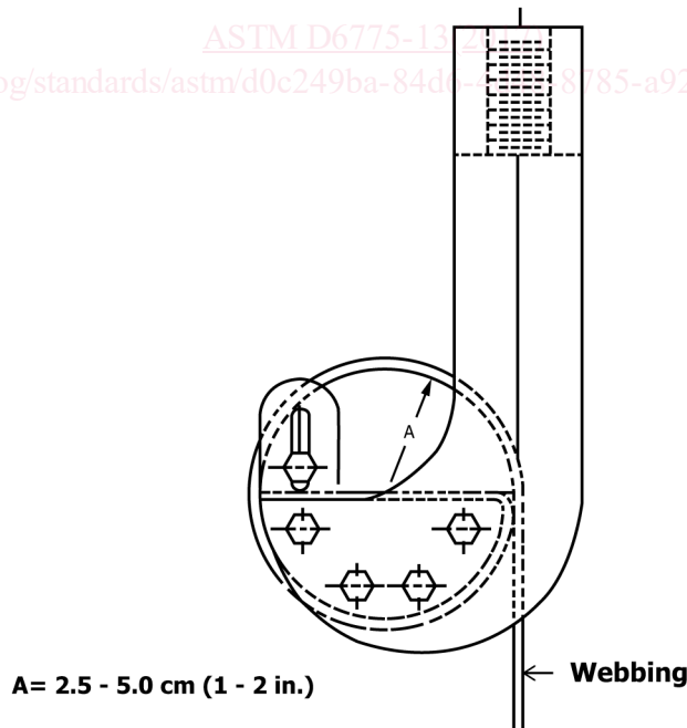
TEST JAWS FOR HIGH STRENGTH TEXTILES
