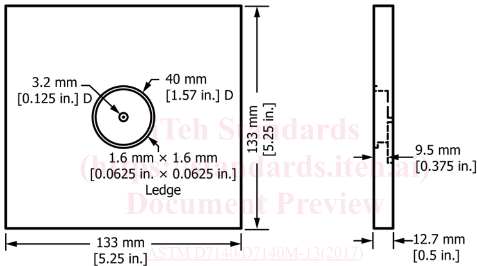
FIG. 2 Calorimeter Placement
