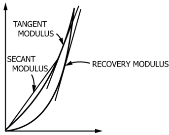
FIG. 2 Relationship Between Tangent, Secant, and Recovery Moduli for a Single Loading and Unloading Cycle
