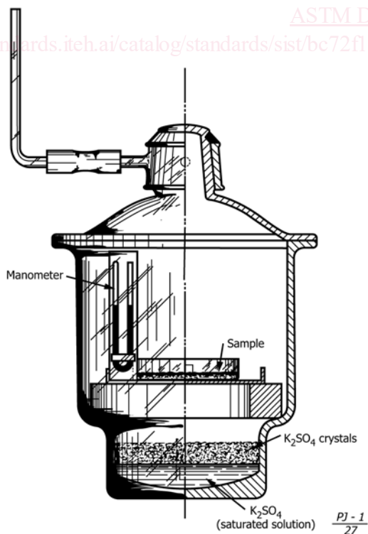
FIG. 1 Vacuum-Type Desiccator
