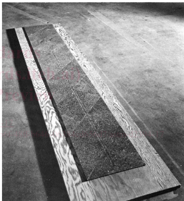
FIG. 7 Wood-Based Finish Floor Applied to Plywood with Tile Oriented so that Loaded Caster will Roll Across Corner
