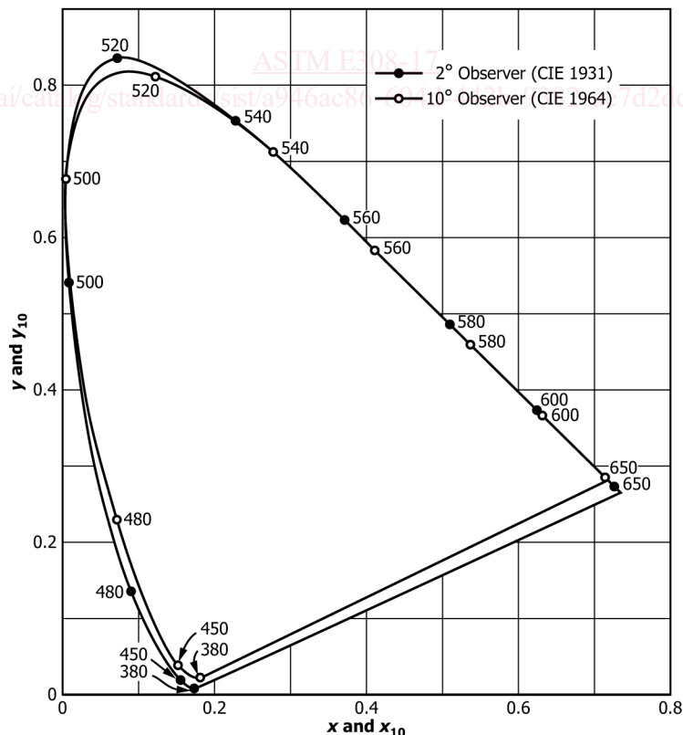
FIG. 1 The CIE 1931 x_{\bar{2}}, y_{\bar{2}} and 1964 x_{10}, y_{10} Chromaticity Diagrams Ref (5) (see Note 2)
