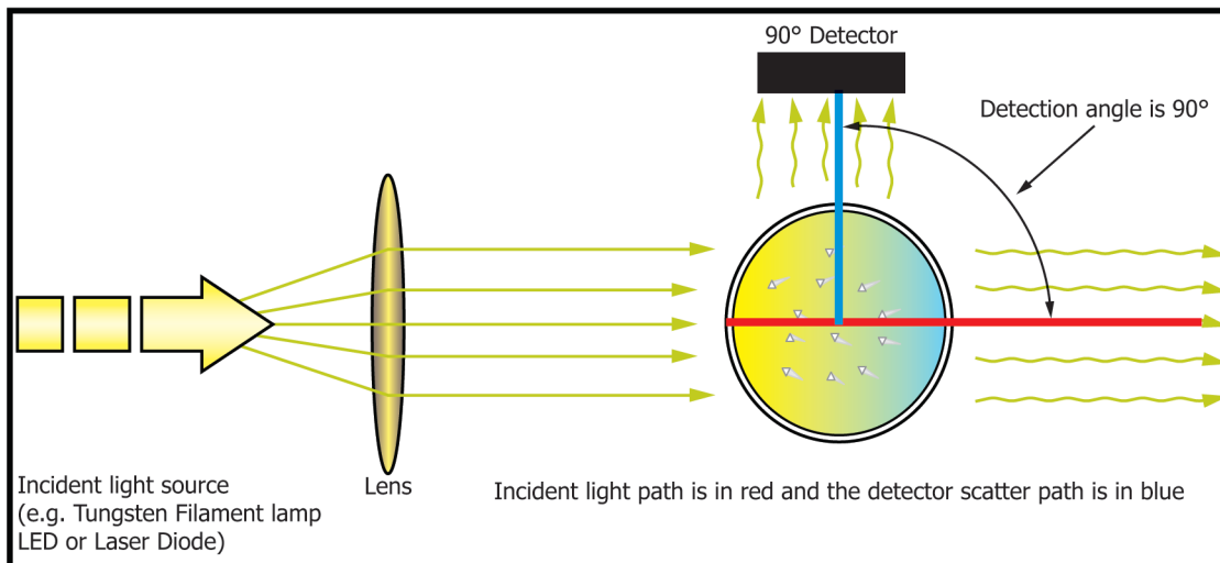
FIG. 1 Typical Nephelometer
