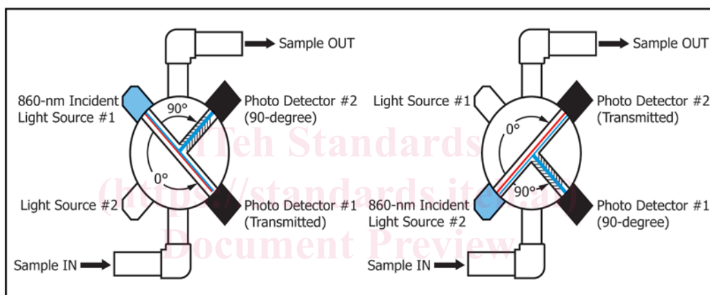
FIG. 3 Ratio Nephelometer (Multiple Beam Design)
