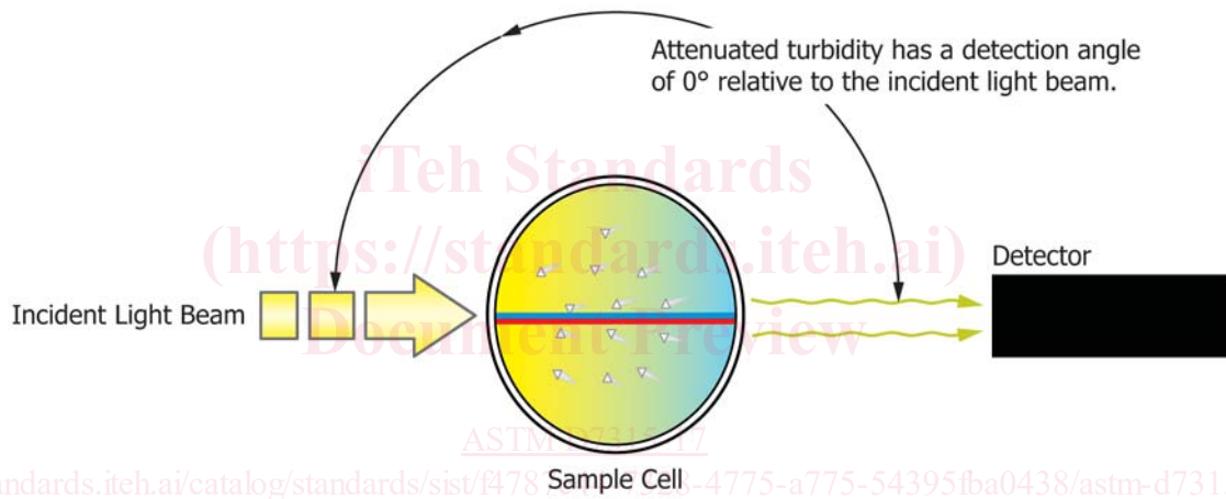
FIG. 5 Technology Diagram of an Attenuation Technology
