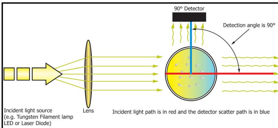
FIG. 1 Typical Nephelometer
