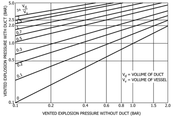
FIG. 1 Influence of Vent Duct Volume on Vented Explosion Peak Pressures (2)
