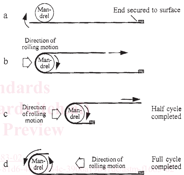
FIG. 1 Bend Cycle
