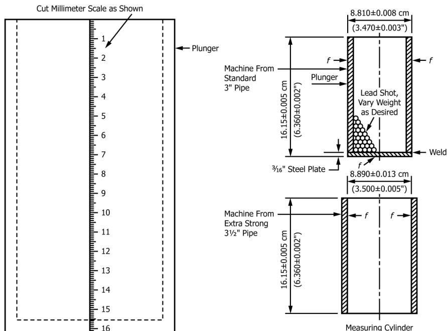
FIG. 3 Apparatus for Apparent Density Test, Method C
