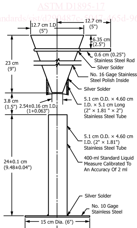
FIG. 2 Apparatus for Apparent Density Test, Method B
