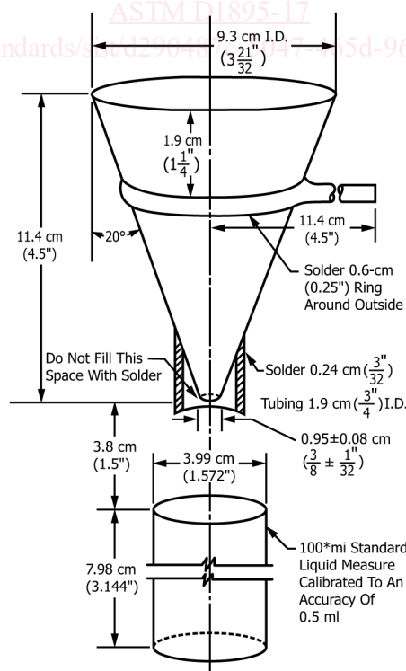
FIG. 1 Apparatus for Apparent Density Test, Method A
